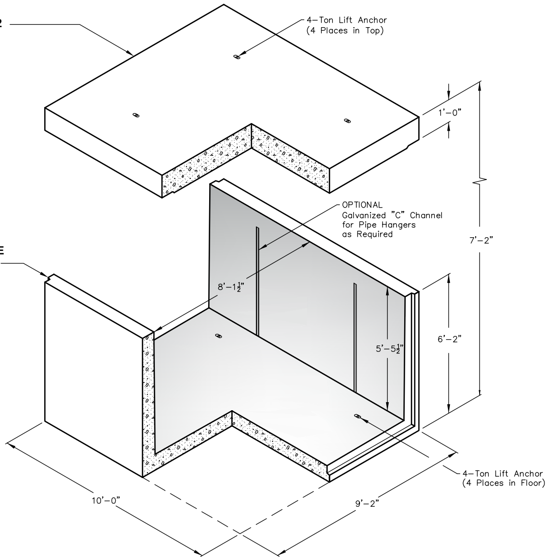
TRENCH TOP No. 8056-TT-12 14,800 lbs.
