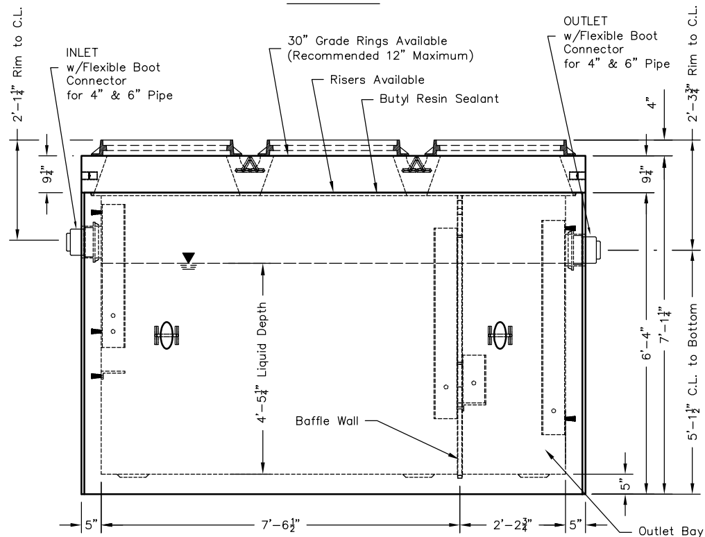
SIDE VIEW
