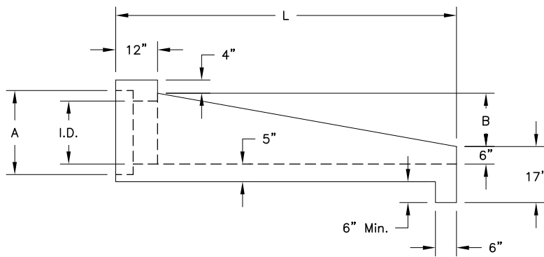
ELEVATION VIEW
