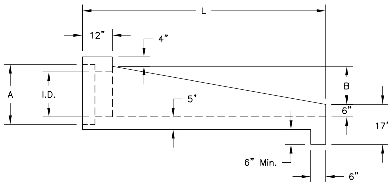
ELEVATION VIEW
