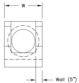
END VIEW
