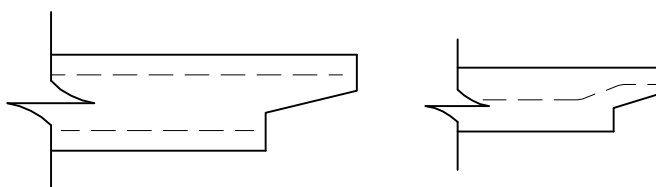
REINFORCEMENT AT BELL ENDS OF PIPES
