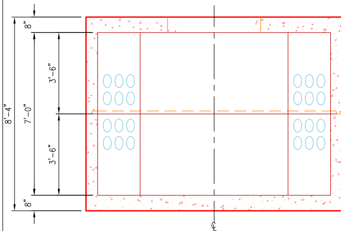
SIDE VIEW SCALE: 1/4" = 1'-0"
