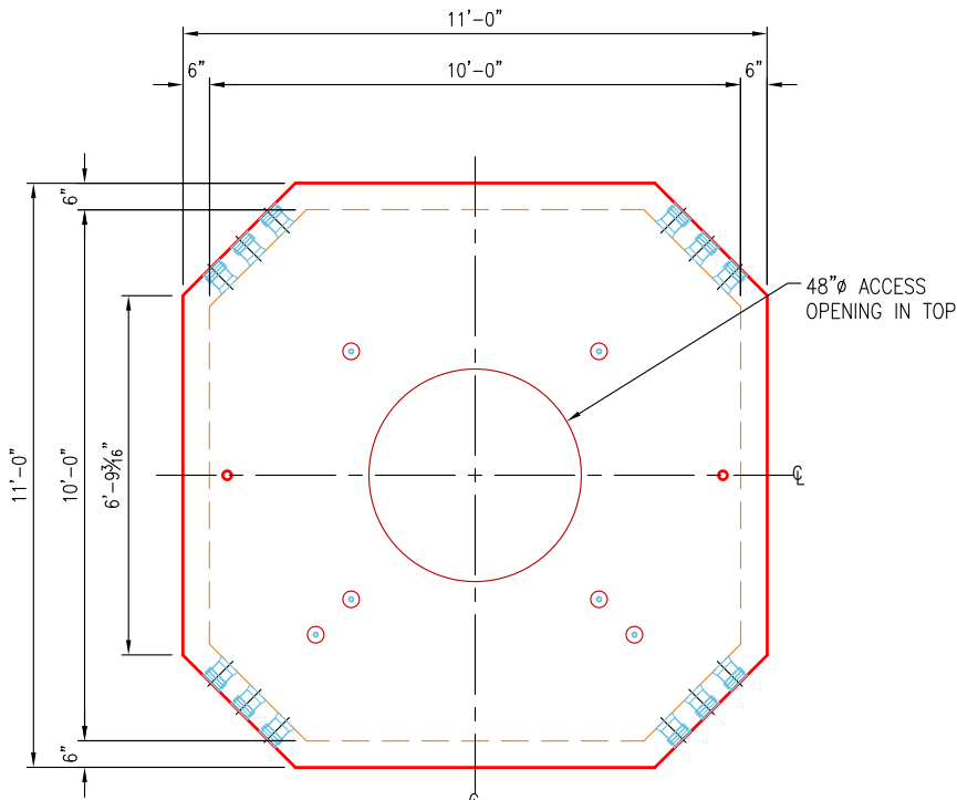
PLAN VIEW SCALE: 1/4" = 1'-0"
