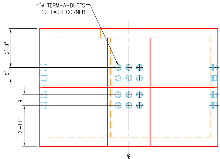
CORNER VIEW SCALE: 1/4" = 1'-0"
