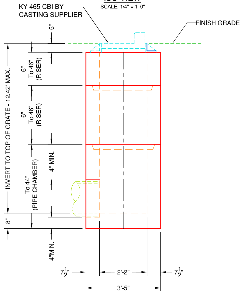
VIEW B
