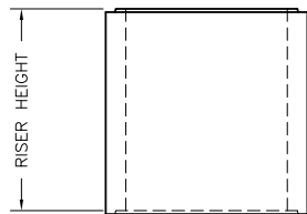
2'-6"x4' CATCH BASIN RISER ELEVATION VIEW
