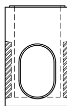
2'-6"x4' CATCH BASIN BASE ELEVATION VIEW
