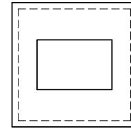
2'-6"x4' CATCH BASIN LID PLAN VIEW 2'x3' OPENING CENTER/OFFSET 18"x48" OPENING CENTER/OFFSET
