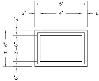
2'-6"x4' CATCH BASIN BASE / RISER PLAN VIEW
