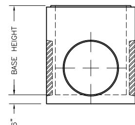
2'-6"x4' CATCH BASIN BASE ELEVATION VIEW
