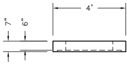
3'x3' CATCH BASIN LID ELEVATION VIEW
