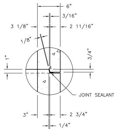
JOINT DETAIL
