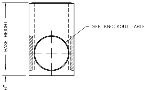
3'x3' CATCH BASIN BASE ELEVATION VIEW
