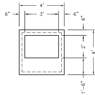
3'x3' CATCH BASIN LID PLAN VIEW 2'x3' OPENING CENTER/OFFSET
