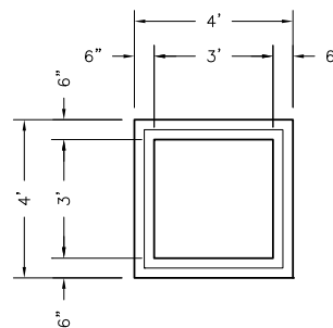
3'x3' CATCH BASIN BASE / RISER PLAN VIEW
